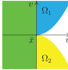
Fig. 3. Subregularity vs Semiregularity
