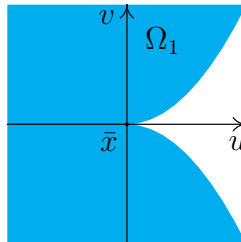
Fig. 4. q -semiregularity
