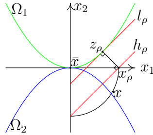
Fig. 2. Subregularity vs \left[\frac{1}{2}\right] -subregularity
